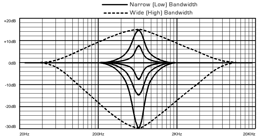
4.24C Parametric Filters
